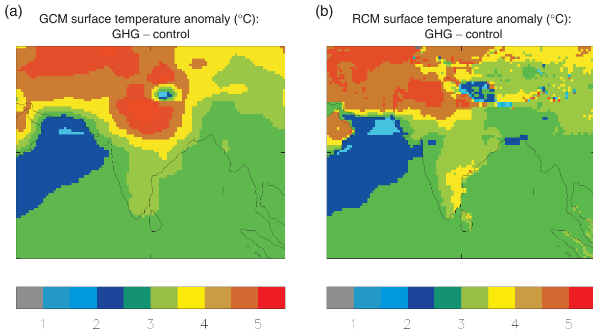
Figure 10.14: Simulated surface air temperature anomaly (°C) for JJA, Indian monsoon region. GHG (2040 to 2060) minus control 20 year average for (a) GCM and (b) RCM. From Hassel and Jones (1999).
