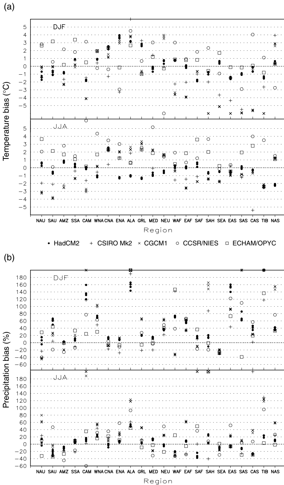
Figure 10.2: Surface temperature biases (in ^{\circ}\text{C} ) and precipitation biases (% of observed) for 1961 to 1990 for experiments using the AOGCMs of CSIRO Mk2, CCSR/NIES, ECHAM/OPYC, CGCM1 (a three-member ensemble) and HadCM2 (a four-member ensemble) with historical forcing including sulphates (further experimental details are in Table 9.1). Regions are as indicated in Figure 10.1 and observations are from New et al. (1999a,b). (a) surface air temperature, (b) precipitation (from Giorgi and Francisco, 2000b).
